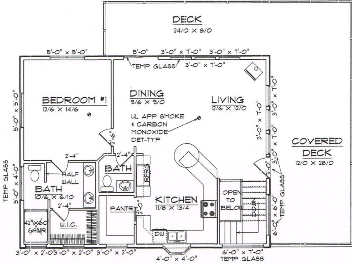
2ND FLOOR LAYOUT SCALE: 1/8" = 1'-0"
