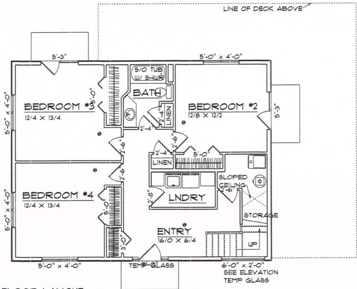
1ST FLOOR LAYOUT SCALE: 1/8" = 1'-0"
