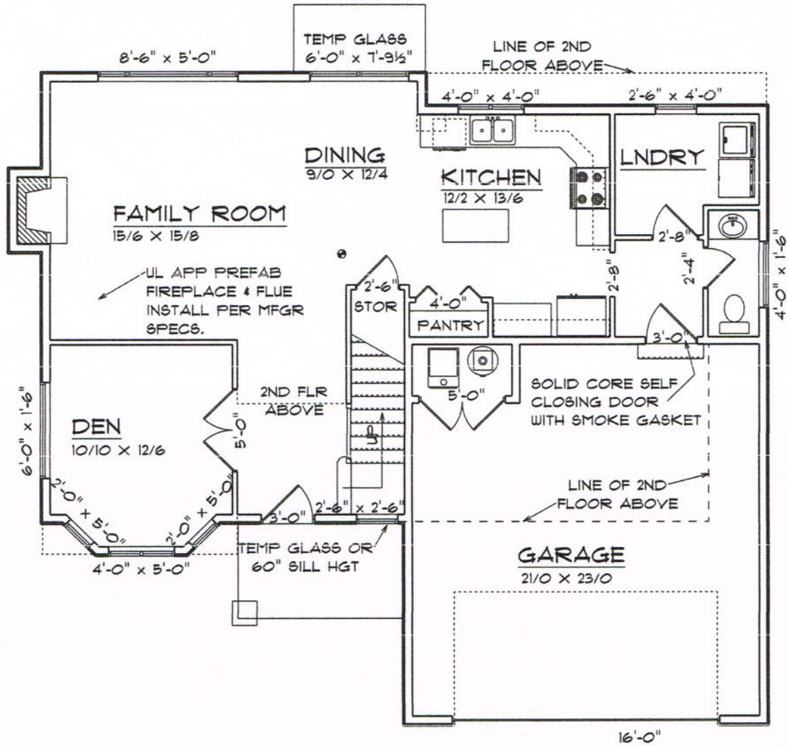
1ST FLOOR LAYOUT SCALE: 1/8" = 1'-0"
