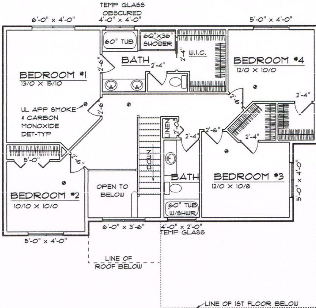
2ND FLOOR LAYOUT SCALE: 1/8" = 1'-0"
