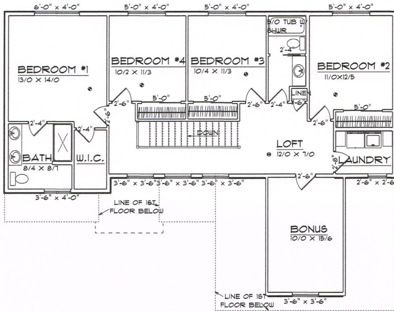
2ND FLOOR LAYOUT SCALE: 1/8" = 1'-0"
