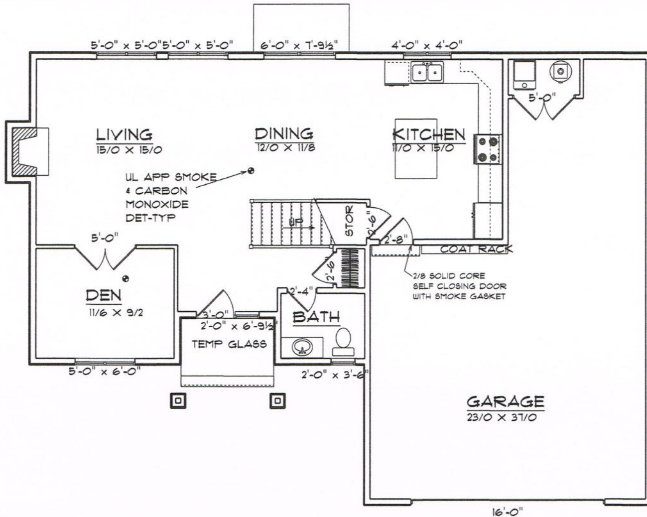
1ST FLOOR LAYOUT SCALE: 1/8" = 1'-0"
